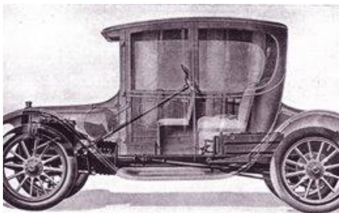
RIGHT VIEW OF WOODS DUAL-POWER CAR, SHOWING LOCATION OF SOURCES OF POWER Courtesy of Woods Motor Vehicle Company, Chicago, Illinois
