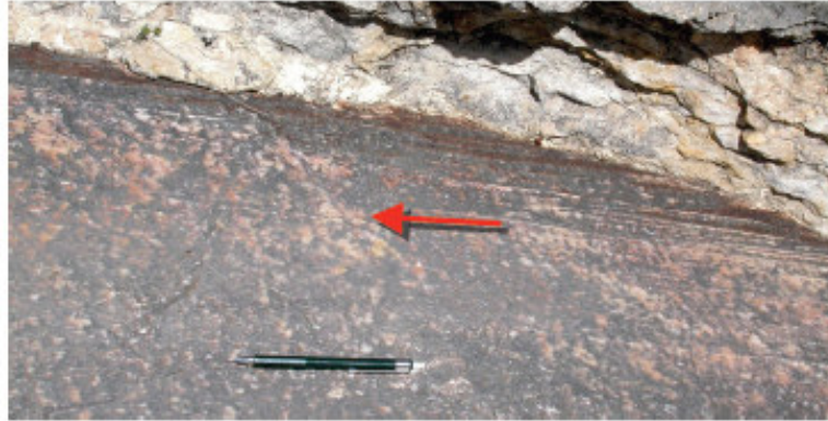
• Fault striations ( Striemung )
